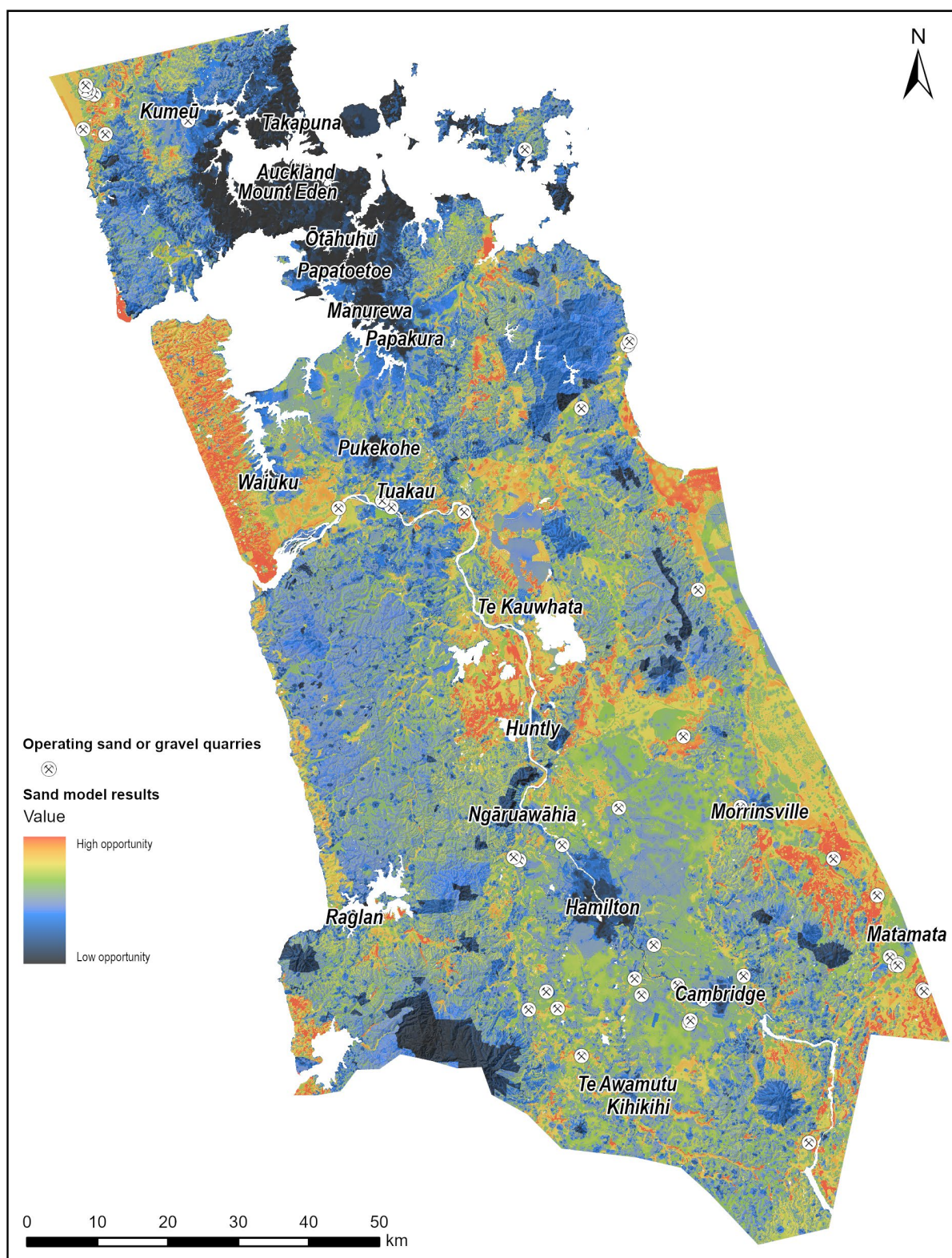
Figure 3.4 Spatial modelling results for sand material from the combined predictive component maps of source rocks, land use, feasibility and sensitivity data using fuzzy logic modelling. This represents Level 3 of the aggregate opportunity modelling process. Maps are scaled and coloured from the resulting fuzzy logic spatial model values that represent low aggregate opportunity (black) to high aggregate opportunity (red). This map is presented at a larger scale as part of Appendix 5.
