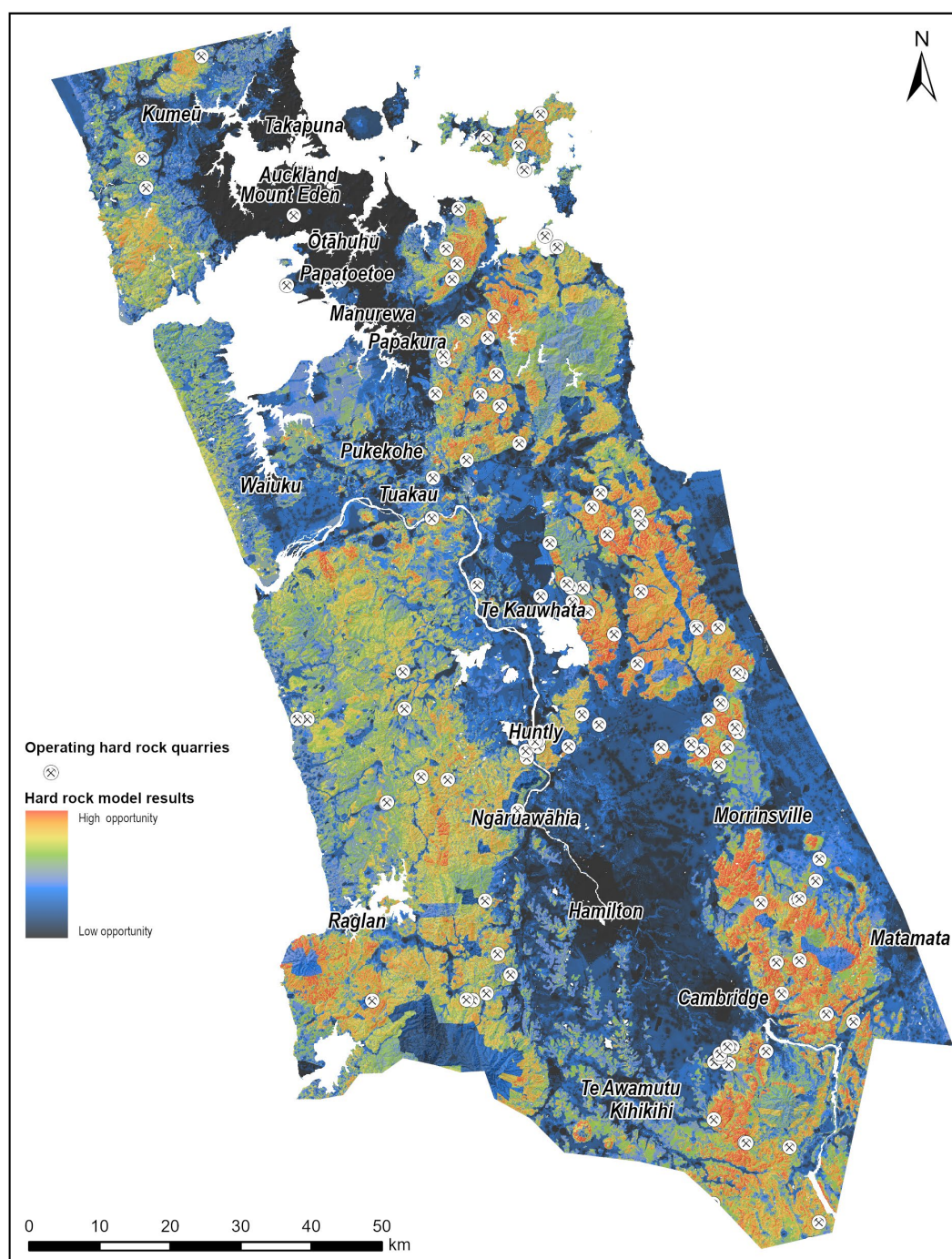
Figure 3.2 Spatial modelling results for hard rock material from the combined predictive component maps of source rocks, land use, feasibility and sensitivity data using fuzzy logic modelling. This represents Level 3 of the aggregate opportunity modelling process. Maps are scaled and coloured from the resulting fuzzy logic spatial model values that represent low aggregate opportunity (black) to high aggregate opportunity (red). This map is presented at a larger scale as part of Appendix 5.
