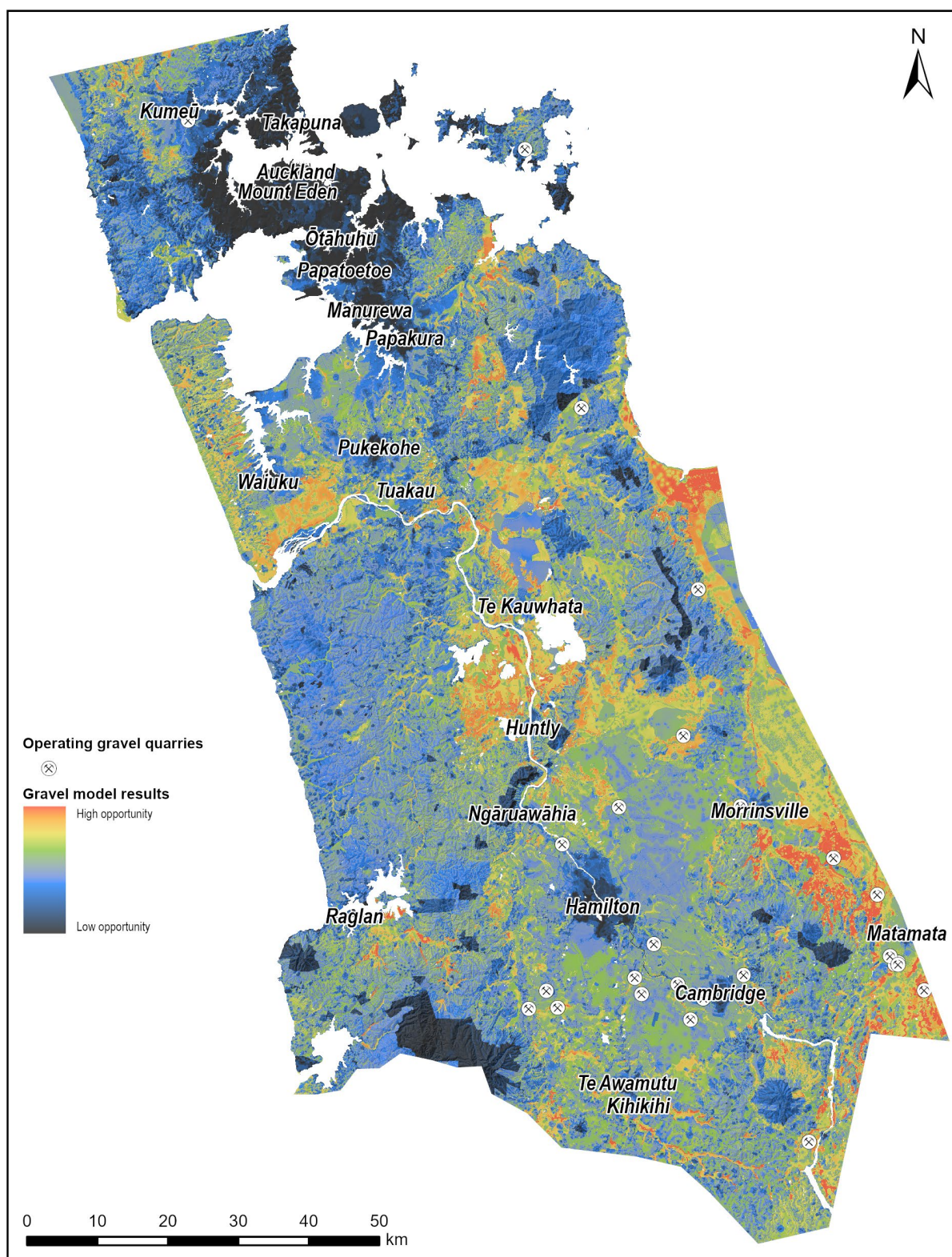
Figure 3.3 Spatial modelling results for gravel material from the combined predictive component maps of source rocks, land use, feasibility and sensitivity data using fuzzy logic modelling. This represents Level 3 of the aggregate opportunity modelling process. Maps are scaled and coloured from the resulting fuzzy logic spatial model values that represent low aggregate opportunity (black) to high aggregate opportunity (red). This map is presented at a larger scale as part of Appendix 5.
