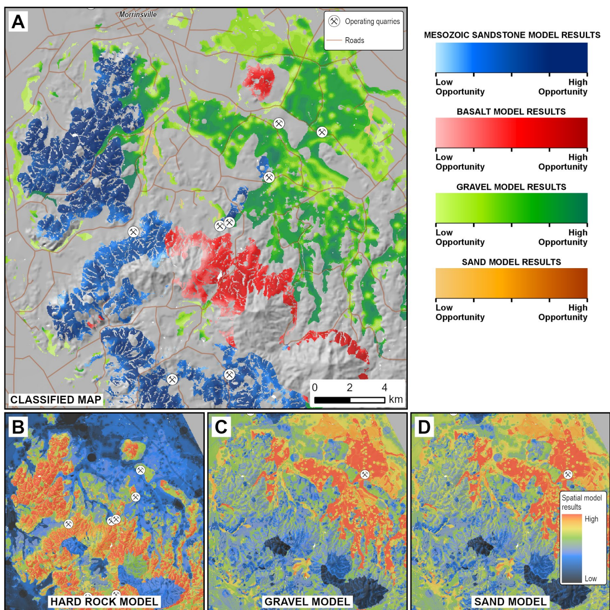
Figure 3.5 Example of an aggregate opportunity model (A) created from spatial model maps for an area between Cambridge and Morrinsville. Mapped data are derived from the Level 3 spatial modelling results (panels B, C and D) and reduced to only values above a significance threshold that represent areas with aggregate opportunity. Model areas above the threshold are grouped and coloured by aggregate type class (see Figure 1.1) and the colour gradient maps show low to high aggregate opportunity.
