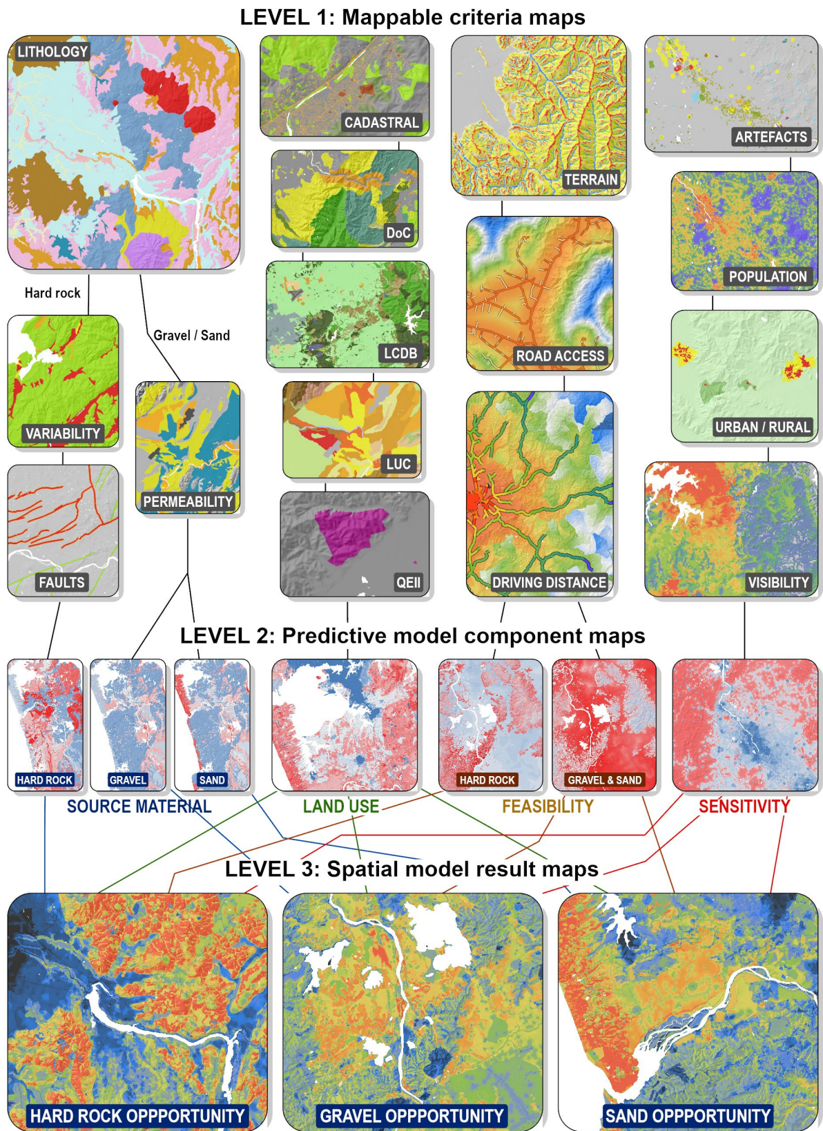
Figure 3.1 Overview of the spatial modelling process for aggregate opportunity modelling and examples of datasets used in this study. Mappable criteria outputs were combined to represent the predictive model components which were then combined to create the final spatial model result maps. Data combination varies for hard rock, gravel and sand models, where the source rocks and terrain maps vary for the different models. Representations of data for the whole study area for each panel in this figure are available in Appendices 3, 4 and 5 of this report.
