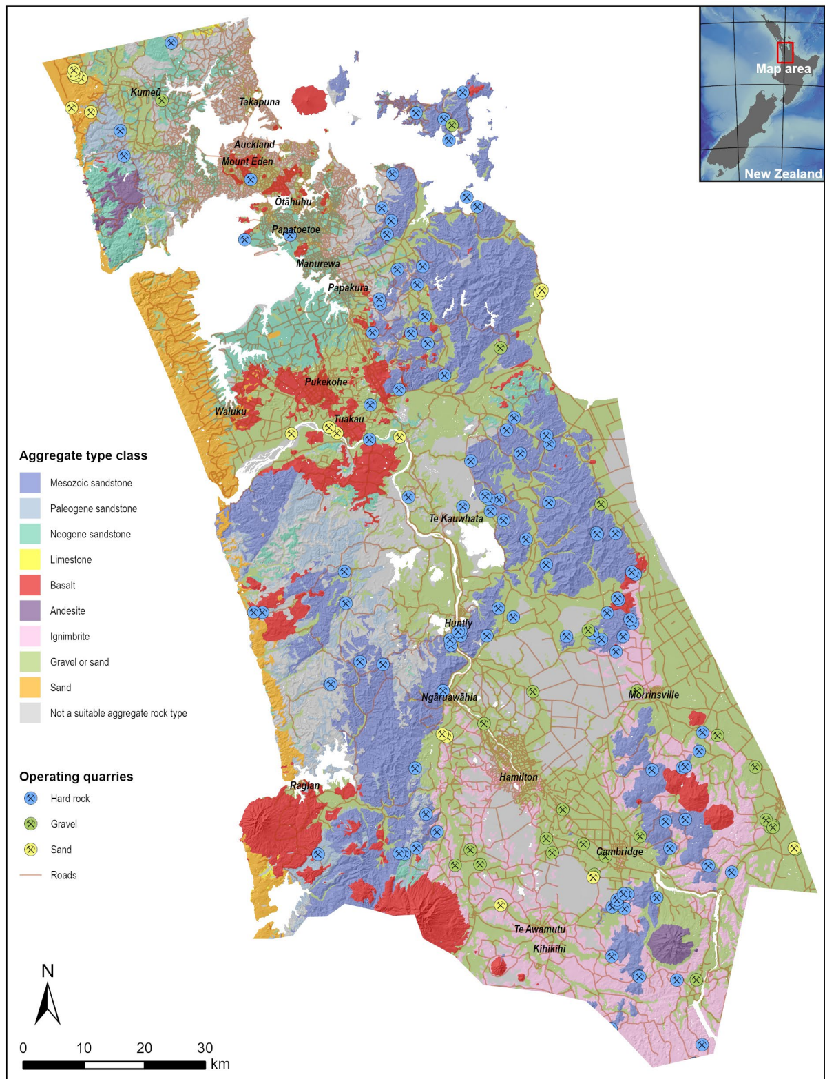
Figure 1.1 Map of aggregate type classes and the extent of the modelled area in the southern Auckland area. Aggregate type class is based on interpretation of regional geological mapping (unit map name, description, main and sub-rock types, and age [Heron 2023]).
