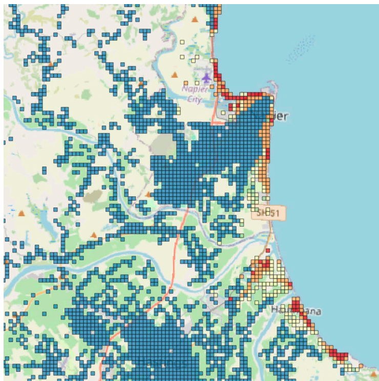
Figure 2.6 Example of estimated average annual loss (AAL) per grid cell for electricity sector from tsunamis. Red colours are higher AAL and blue colours are lower AAL.
