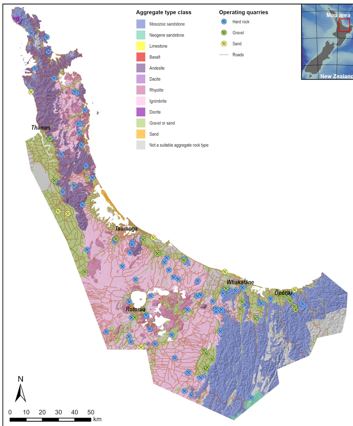
Figure 1.1 Map of aggregate type classes and the extent of the modelled area in the Bay of Plenty area. Aggregate type class is based on interpretation of regional geological mapping (unit map name, description, main and sub-rock types, and age [Heron 2023]).
