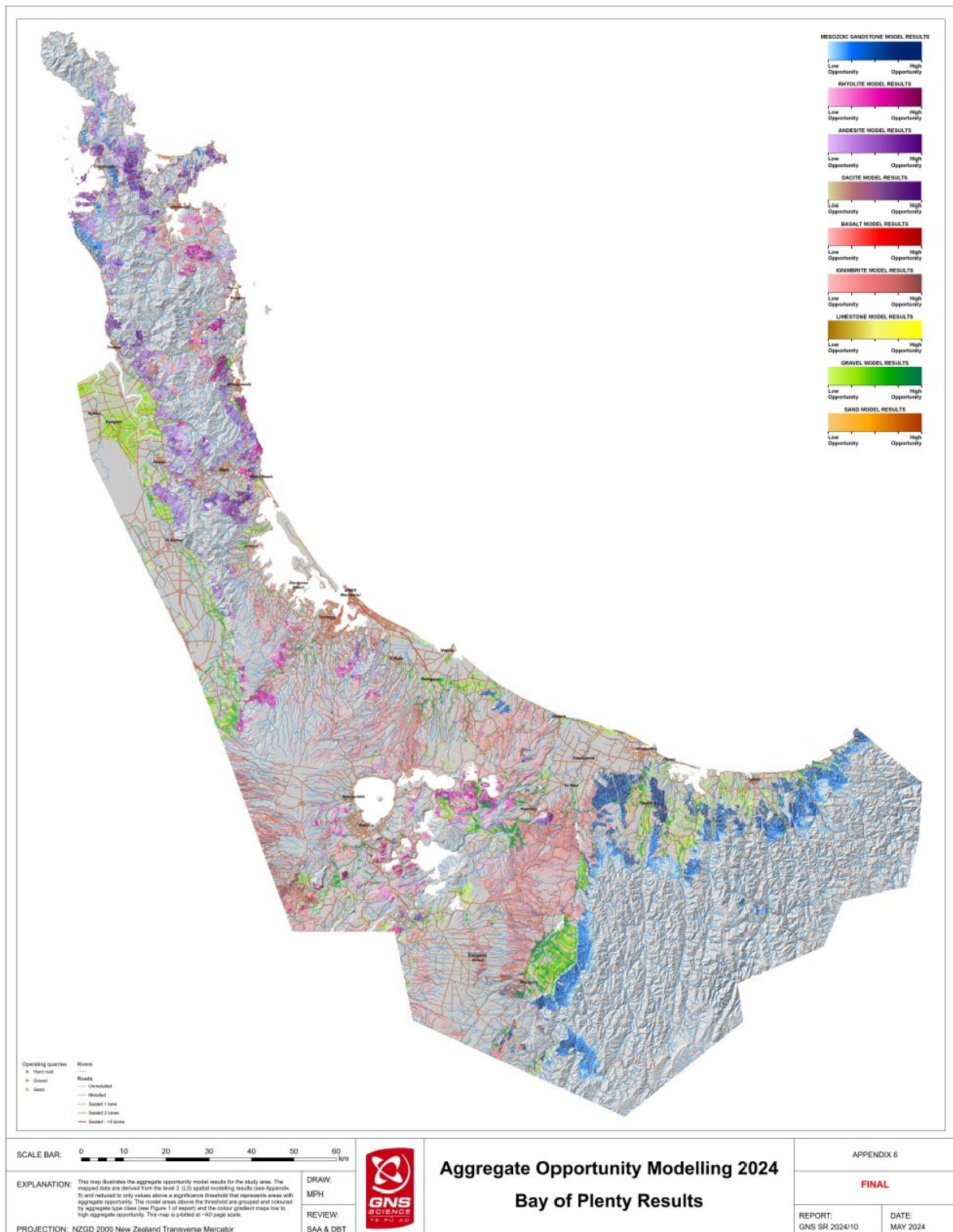
Figure 3.6 Illustration of aggregate opportunity model results poster for the Bay of Plenty area. Colours represent areas above the significance threshold for each aggregate-type class and are colour graded from low to high aggregate opportunity. This map is available in more detail at a larger A0 page-scale as part of Appendix 6.
