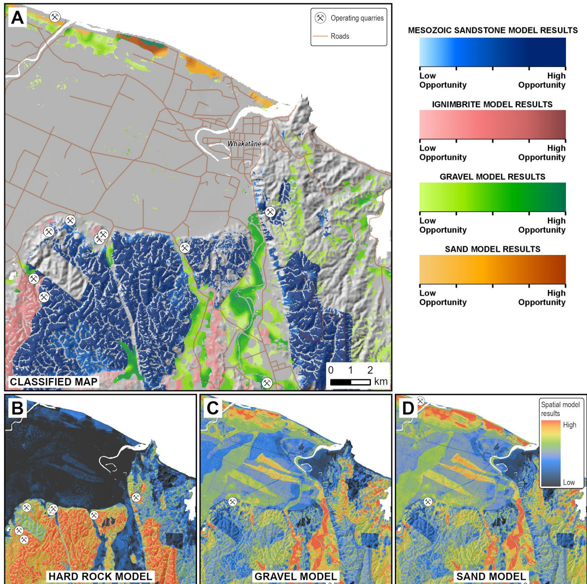
Figure 3.5 Example of an aggregate opportunity model (A) created from spatial model maps (B–D) for the Whakatāne area of the Bay of Plenty. Mapped data are derived from the Level 3 spatial modelling results and reduced to only values above a significance threshold that represent areas with aggregate opportunity. Model areas above the threshold are grouped and coloured by aggregate type class (see Figure 1.1) and the colour gradient maps show low to high aggregate opportunity.
